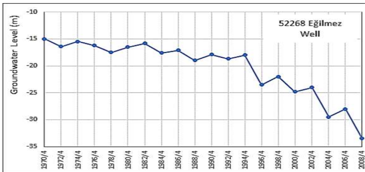
Figure. 7A. Long-term groundwater level changes around Karapınar: Eğilmez well (No. 52268). Well location is given in Figure 5.
