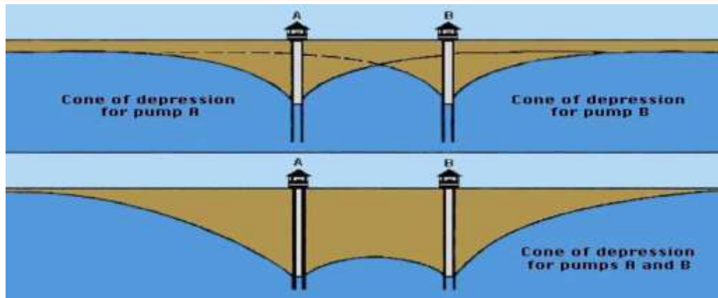
Figure 2. Cone of depression, area of influence, and well interference.
