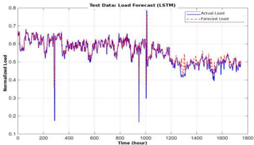
Figure 2. Full test-period load forecast (actual vs. forecast, normalized scale).
