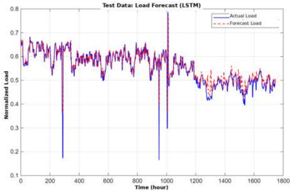
Figure 2. Full test-period load forecast (actual vs. forecast, normalized scale).
