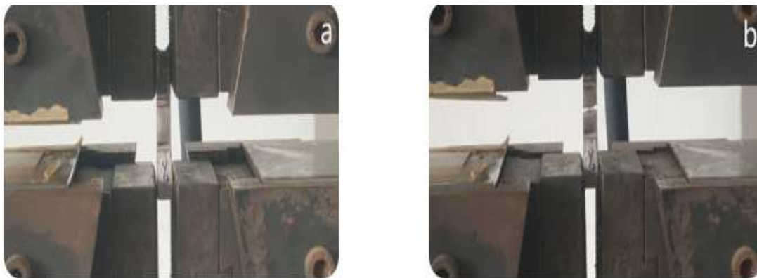
Figure 2. Vertical tensile test setup of the Al/TiB 2 composite samples: (a) the sample fixed between the jaws with marked gauge section at the beginning of the test, and (b) the final fracture appearance occurring at the center of the gauge section at the end of the test
