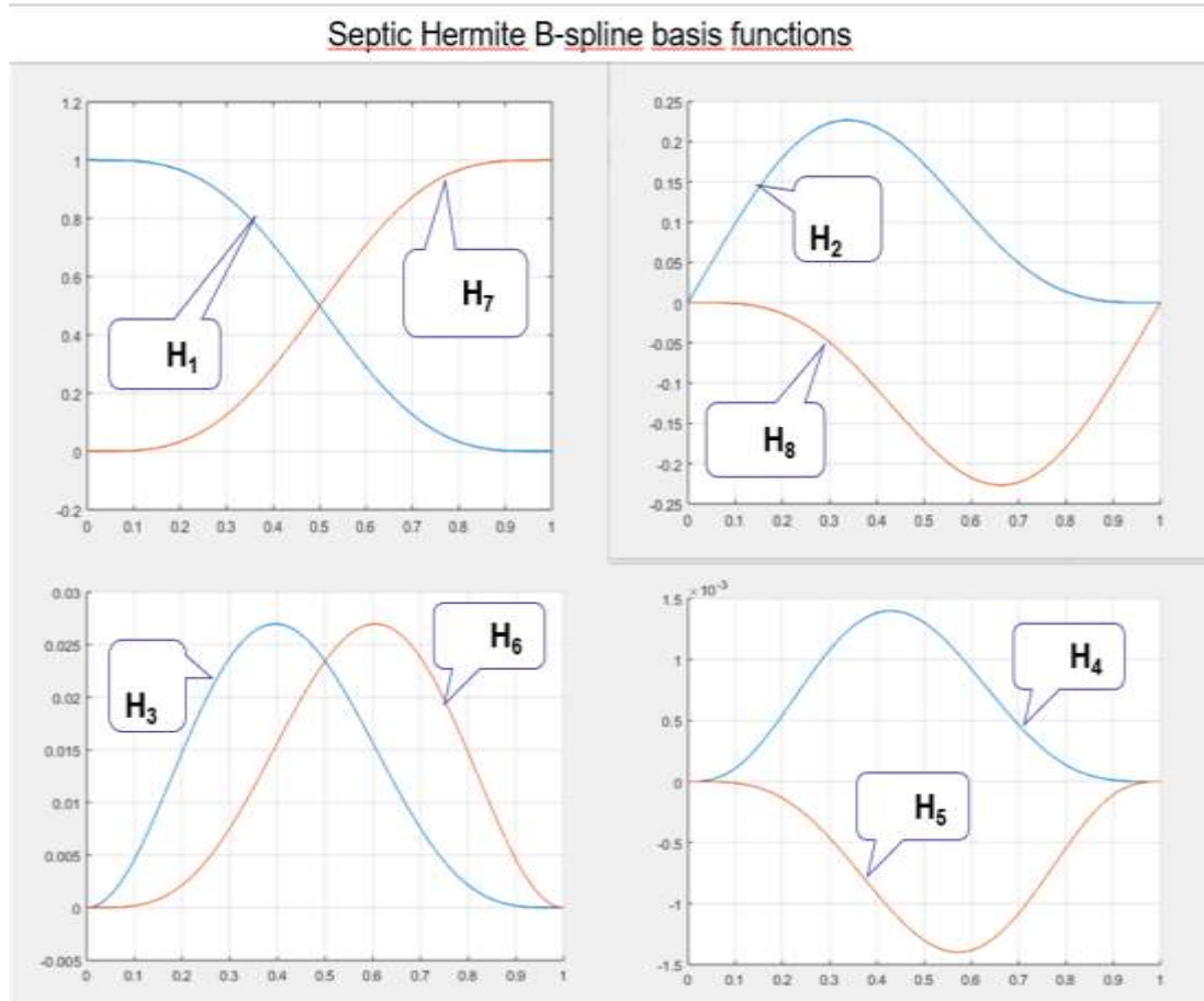
Hermite bases on one element.
