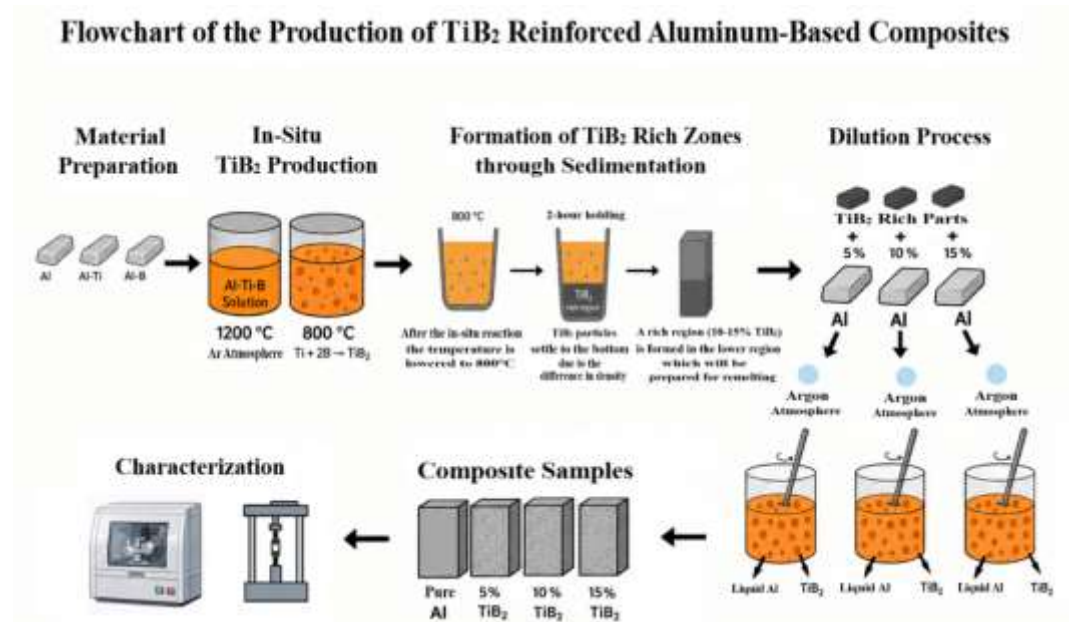
Figure 1. General flowchart of the production process
