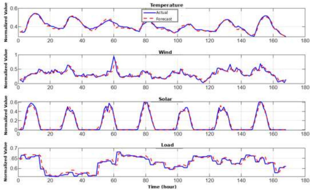
Figure 1. Test-set forecast comparison for the four variables, first week (actual vs. forecast, normalized scale).
