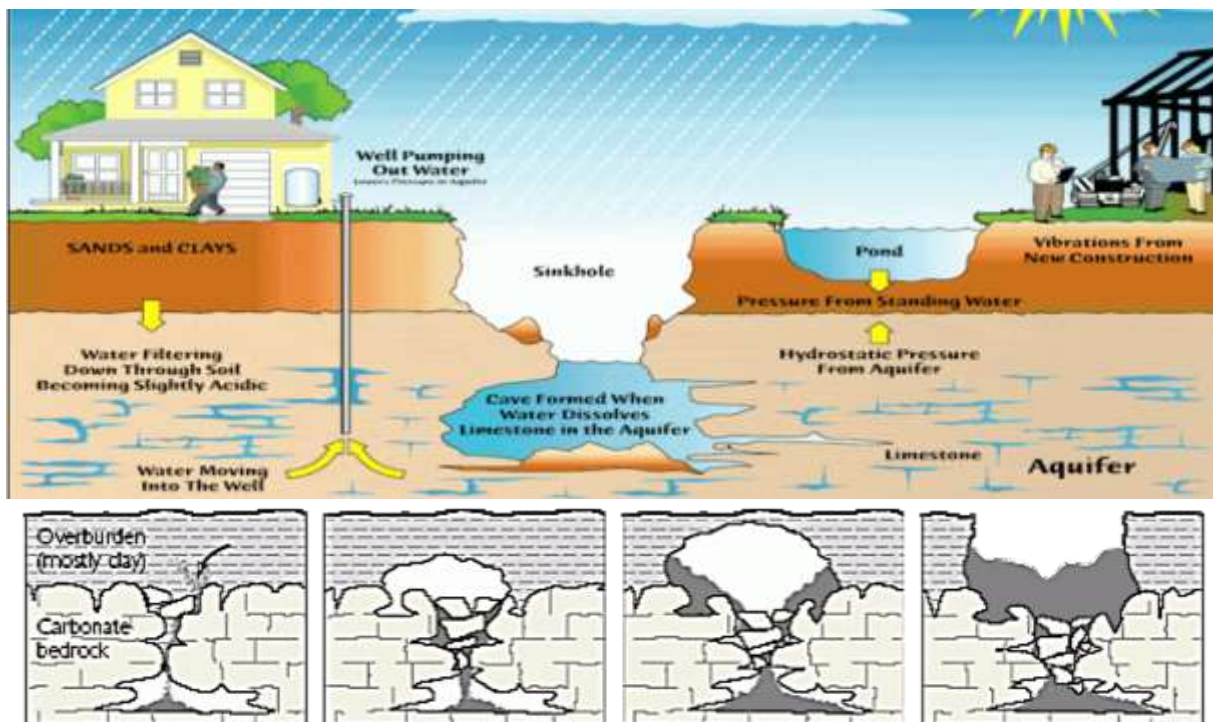
Figure 3. Possible mechanism for sinkhole formation ( http://ga.water.usgs.gov/edu/sinkholes.html )
