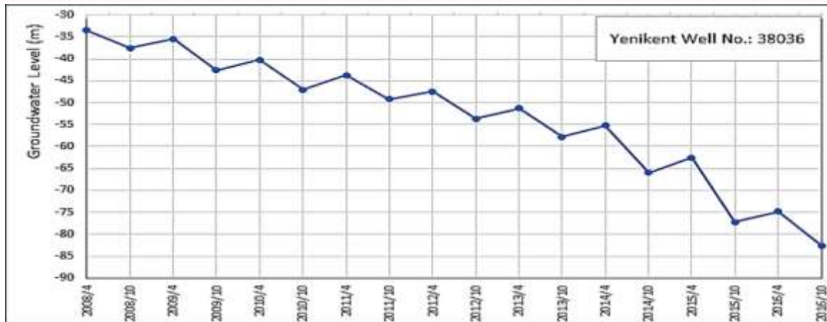
Figure. 7B. Long-term groundwater level changes around Karapınar: Yenikent well (No. 38036). Well location is given in Figure 5.
